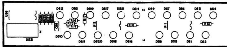
DISPLAY BOARD
