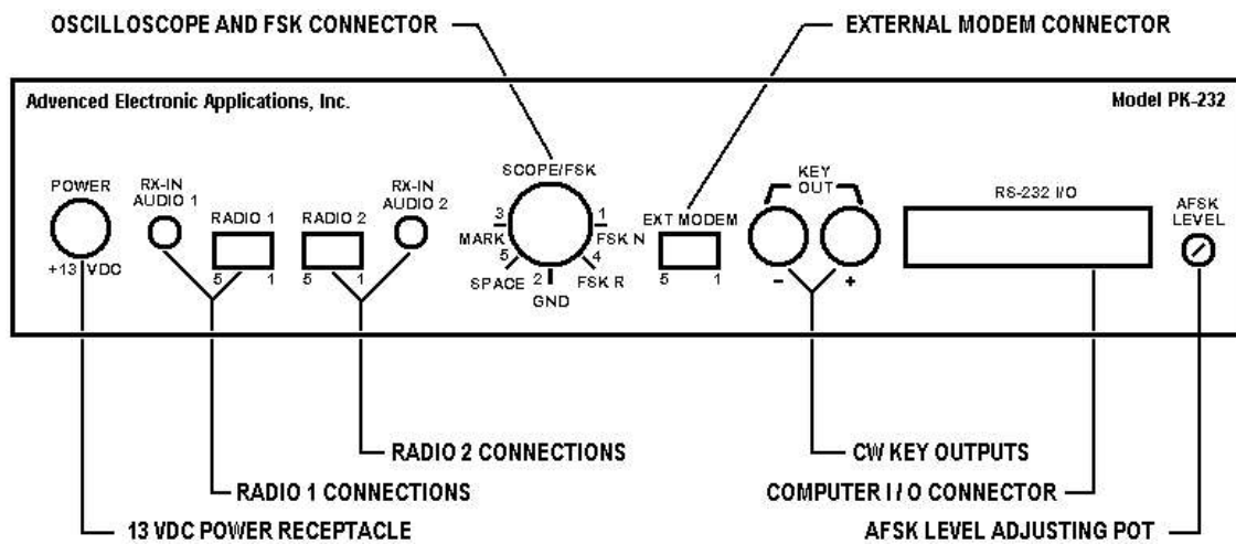
Figure 2-2 PK-232 Rear Panel Connections and Controls
