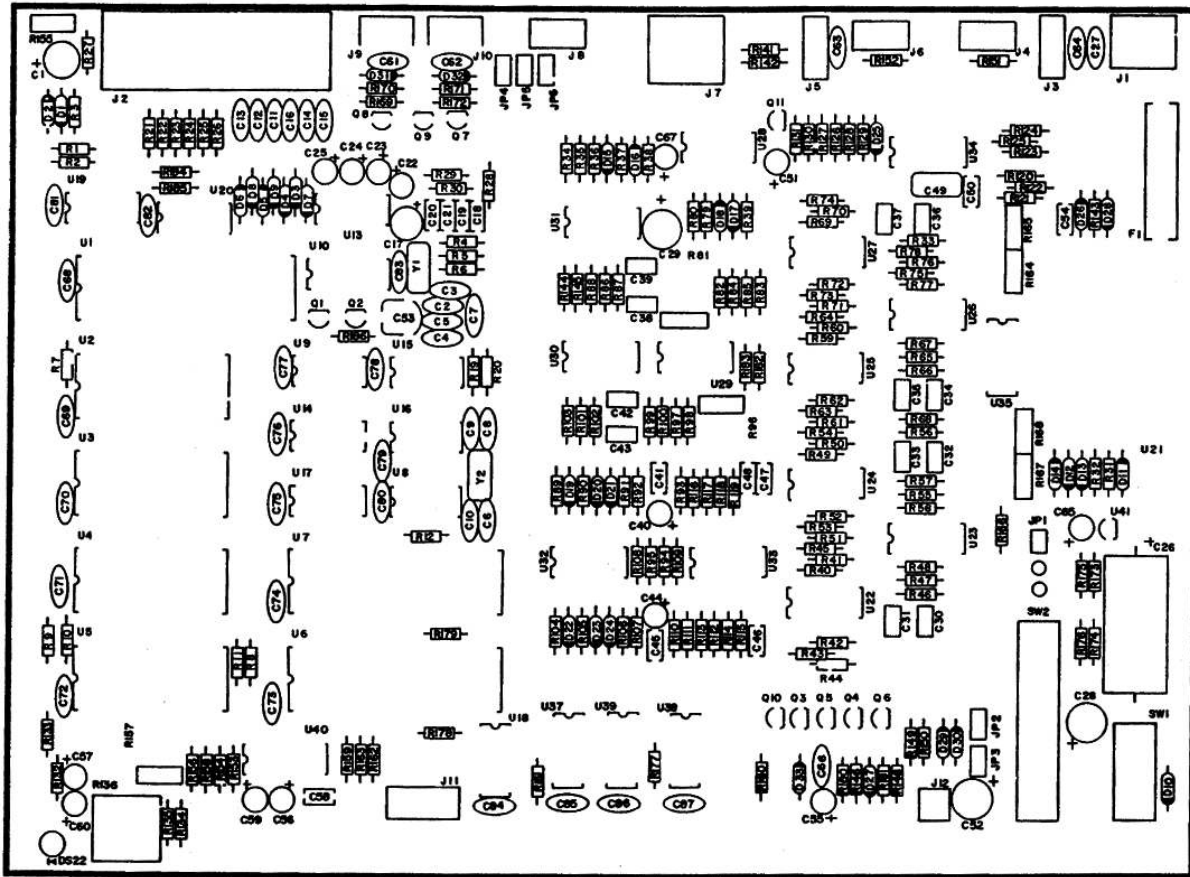
MAIN BOARD
