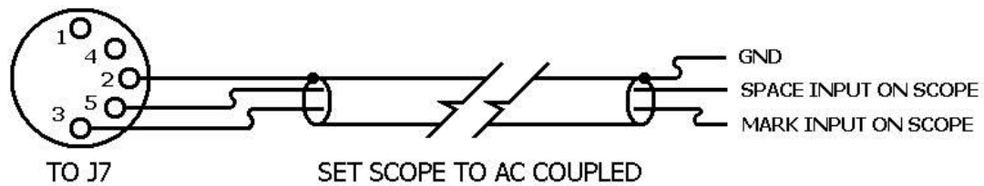
Figure 2-5 Connector J7 Tuning Scope Connections
