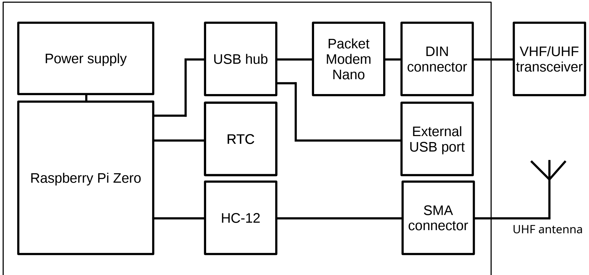
Block diagram: experimental amateur radio data transceiver for old style 1200bps AX.25 (packet radio) and high(er) speed via HC-12 UHF module.
