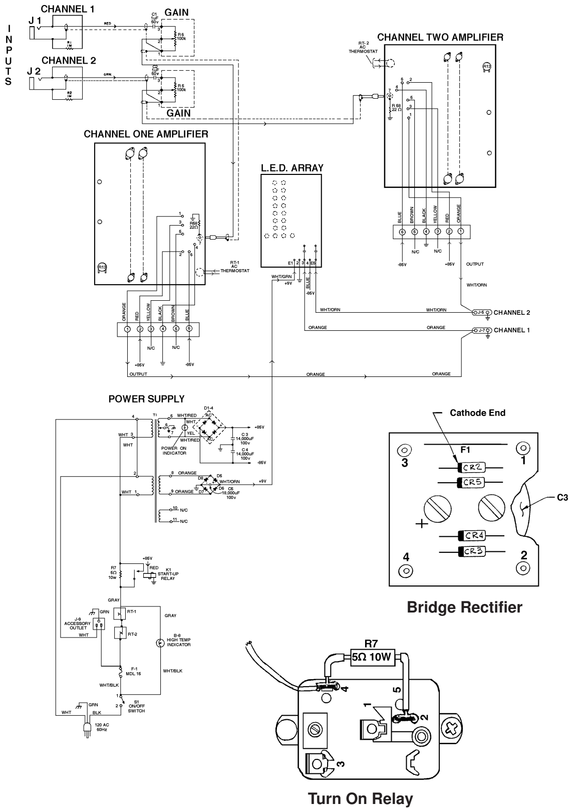
Figure 9. 1801/1800 Block Diagram
